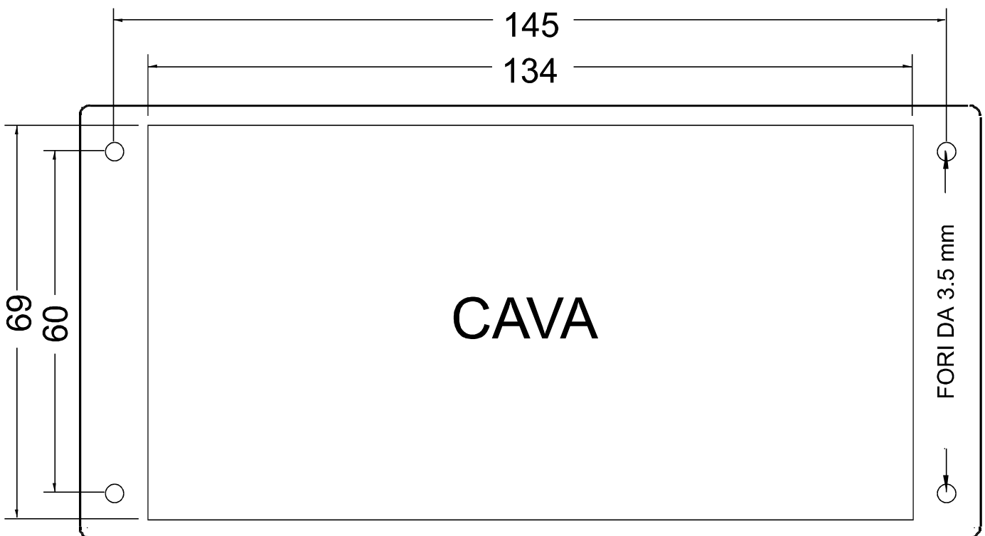
Figure 1.2 - F1-10 panel hole dimension
