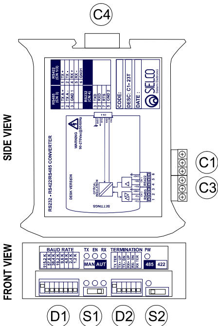
Fig 1 - C1-23T layout
