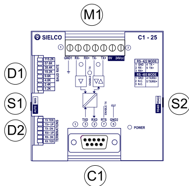
Fig 1 - C1-25- layout
